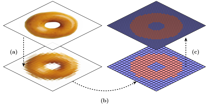
Figure 6: Multiresolution graph cut: (a) Downsample target image. (b) Graph cut is performed a reduced level of our image pyramid. (c) Map solution to original resolution.
