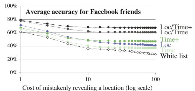
Fig. 5 The average accuracy for the Facebook friends group, under each of the different privacy-setting types, while varying the cost associated with mistakenly revealing a location from c = 1 –100
