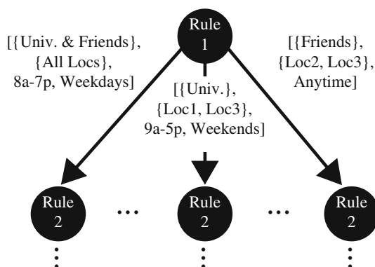
Fig. 2 Part of a search tree for identifying a subject's most accurate privacy policy using Loc/Time+ settings
