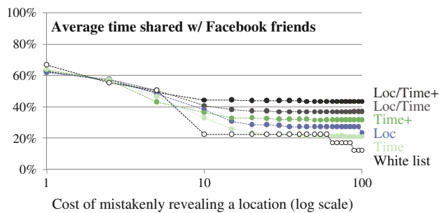
Fig. 7 The average percentage of time shared with the Facebook friends group, under each of the different privacy-setting types, while varying the cost associated with mistakenly revealing a location from c = 1 –100
