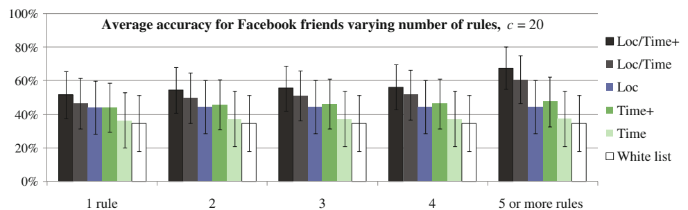
Fig. 8 The average accuracy ( vertical axis ) achieved by each of the different privacy-setting types, for each of the different groups, varying a global limit on the number of rules ( horizontal axis , from 1 to 5 or more) in a policy. We hold constant the cost for
