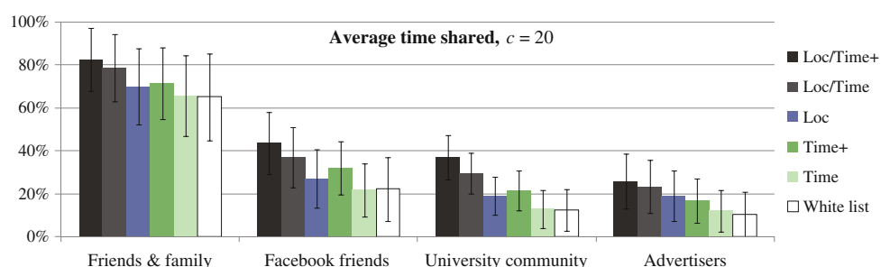
Fig. 6 The average percentage of time shared (bars indicate 95% confidence intervals) with each group under each of the different privacy-setting types. For these results, we hold constant the cost for inappropriately revealing a location at c = 20
